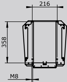
seat mounting
