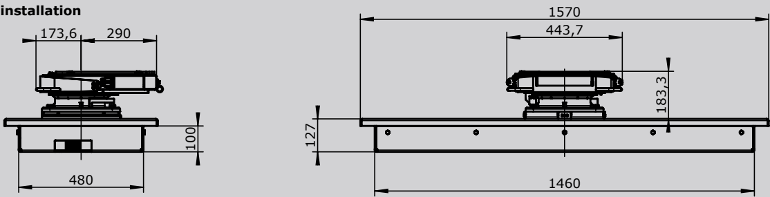
assembly installation
