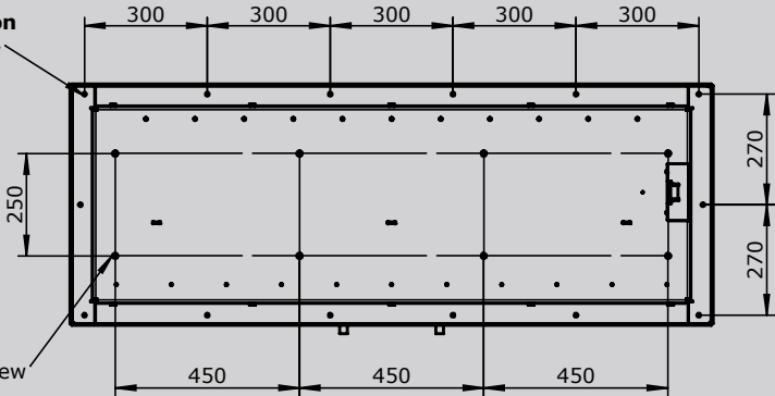
floor mounting
