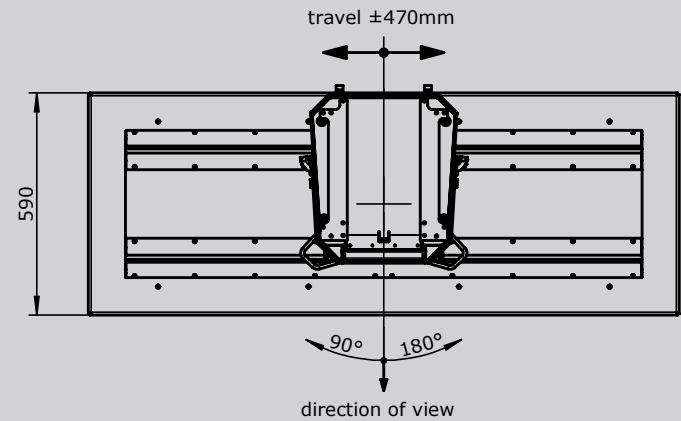
floor mounting
