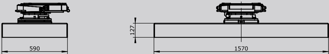
Assembly construction
