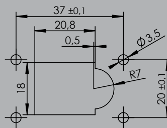
Hole pattern
