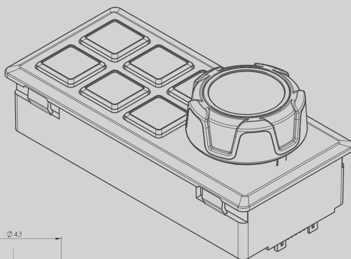
Rotary push-slider
