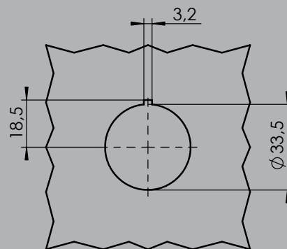
hole pattern with anti-twist
